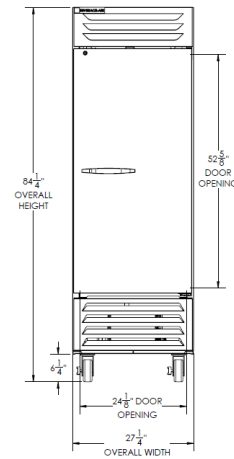
Elevation View
